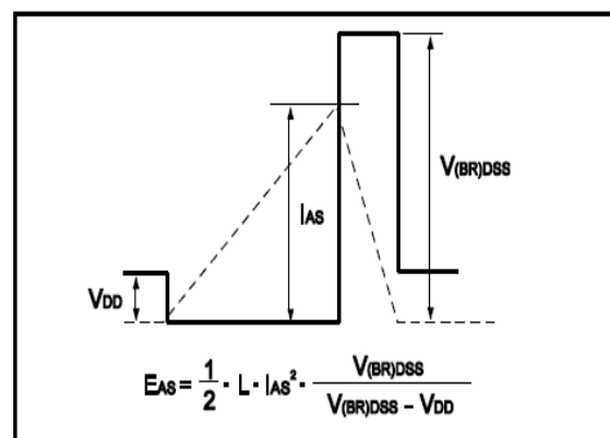
Fig.18 Avalanche Waveform
