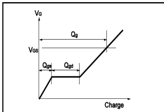
Fig.14 Gate Charge Waveform
